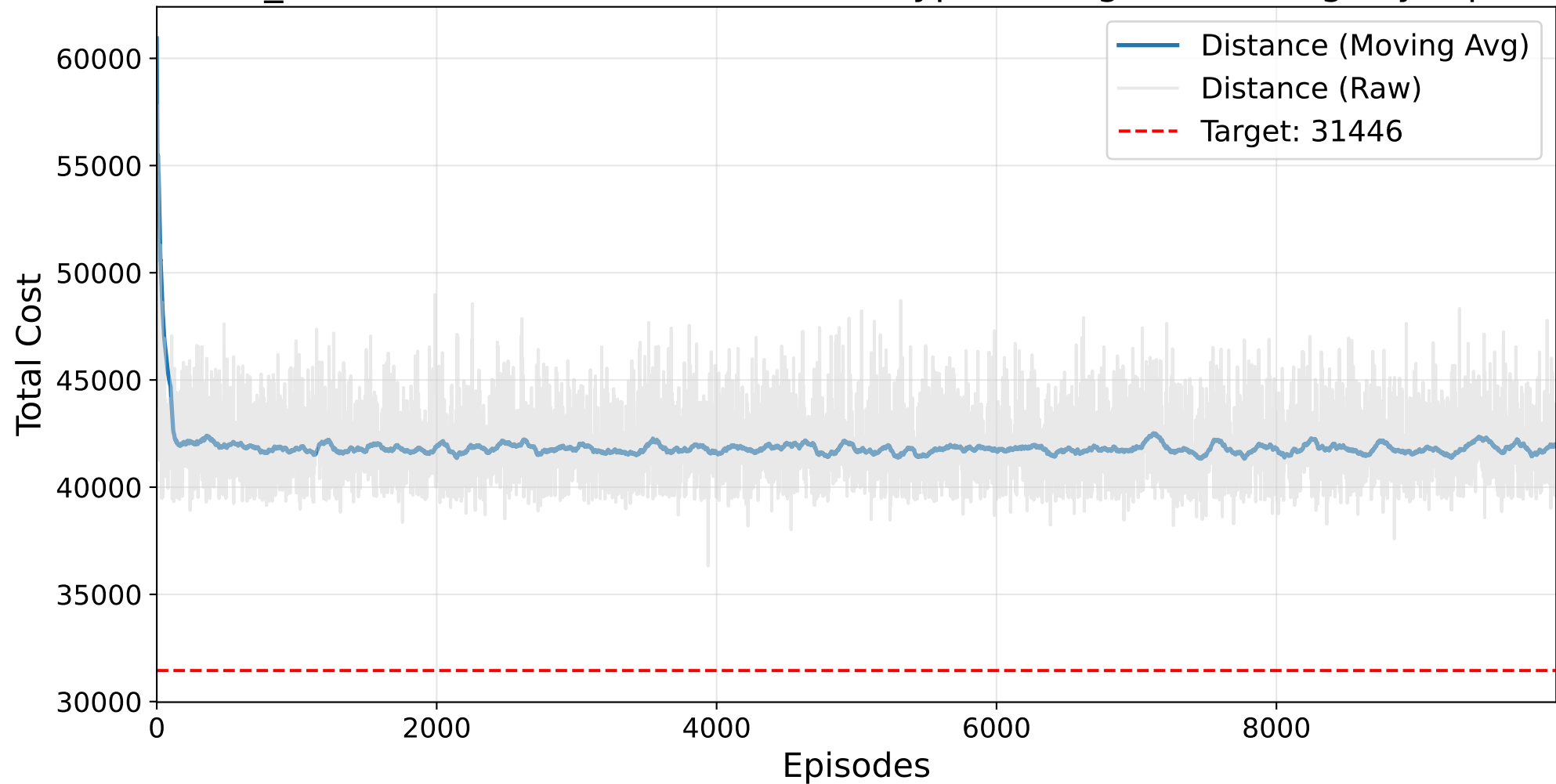
Final NO_BAYESIAN Masked AutoRL-SOP (HyperTuningSK) Training - ry48p.4.sop
